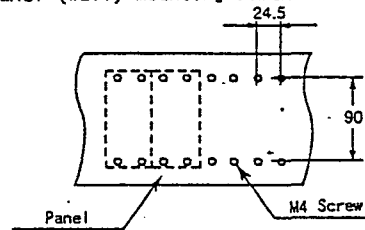
Fig.8 Panel (Wall) Mounting Dimension
