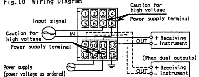
Fig.10 Wiring Diagram
