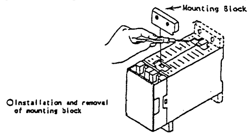
Fig.6 Mounting Block installation and removal
